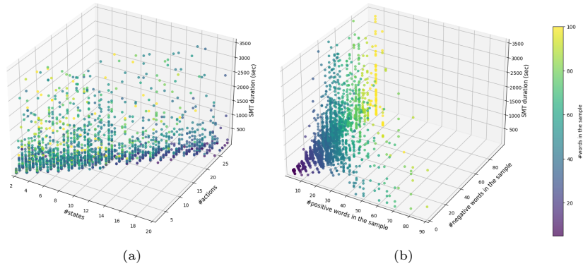
Fig. 6: More plots for SMT duration according to several parameters
