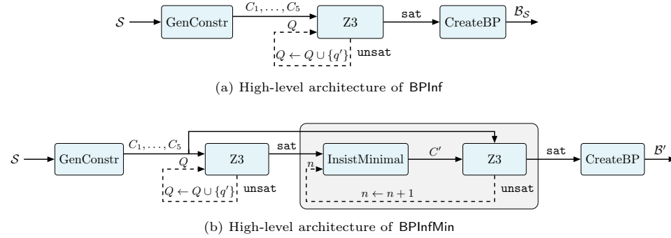
Fig. 3: The high-level architectures of BPInf and BPInfMin .
