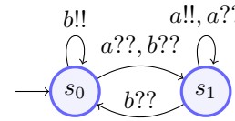
Fig. 1: BP \mathcal{B}_{toy} with 2 states
