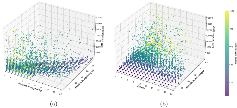
Fig. 5: SMT duration according to several parameters
