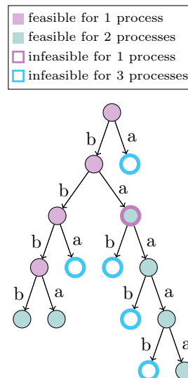
Fig. 2: Tree representing the CS of \mathcal{B}_{toy}
